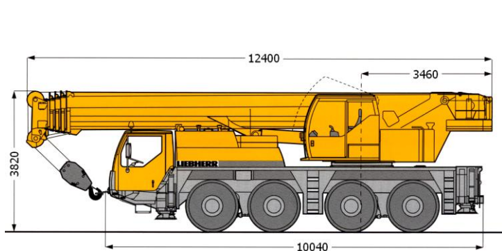
Liebherr LTM 1060/2
